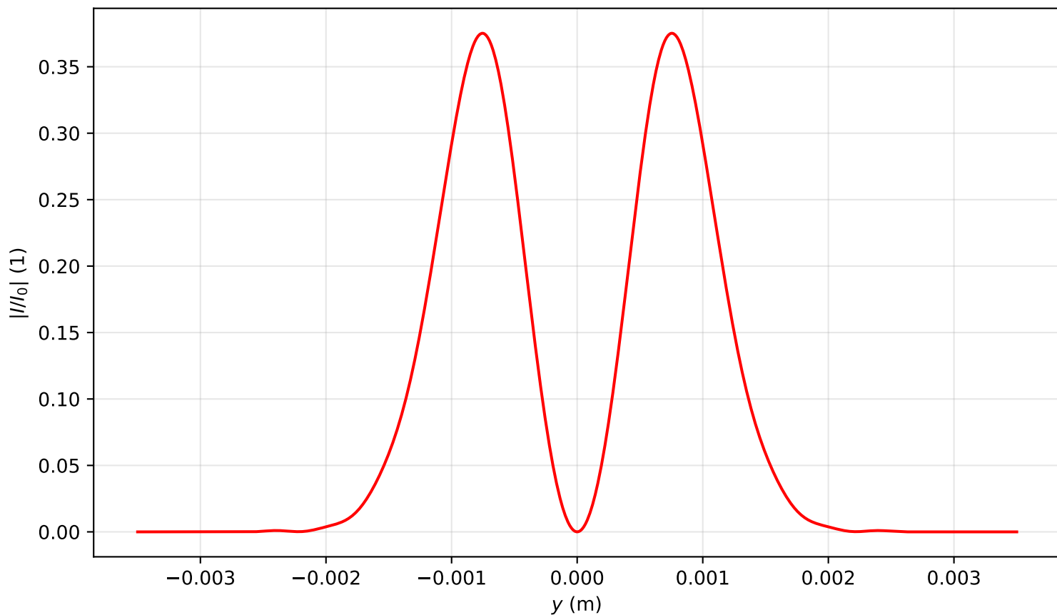
Intensity profile I(x=0, y, z=2.627)/I_0 , P_{in}=2.0P_{cr} , artificial time
